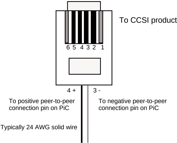
Figure N1-6. RJ11 Modular Plug (6 position - 4 contact) for Twisted Pair Wire
