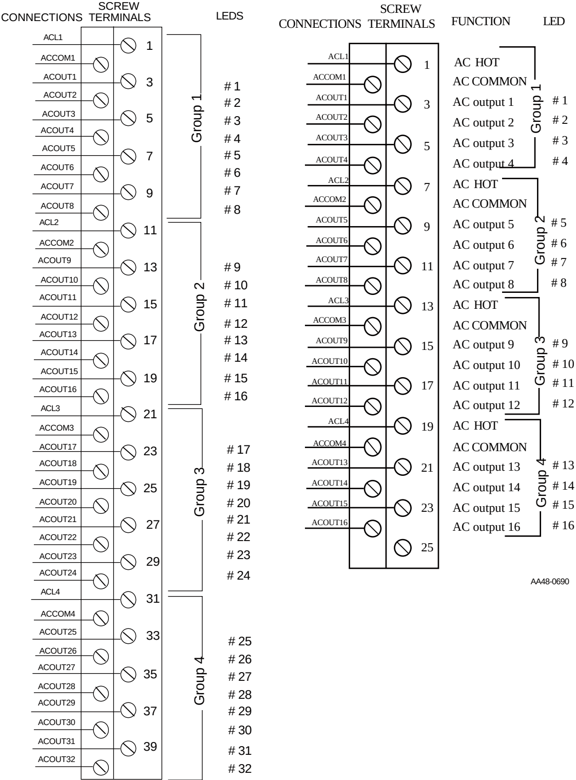
Figure C3-2. Screw Terminal Connector Assignments
