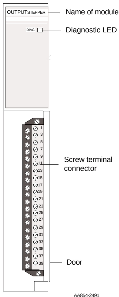
Figure D6-1. OUTPUT STEPPER Module (2, 4, 8 ch)
