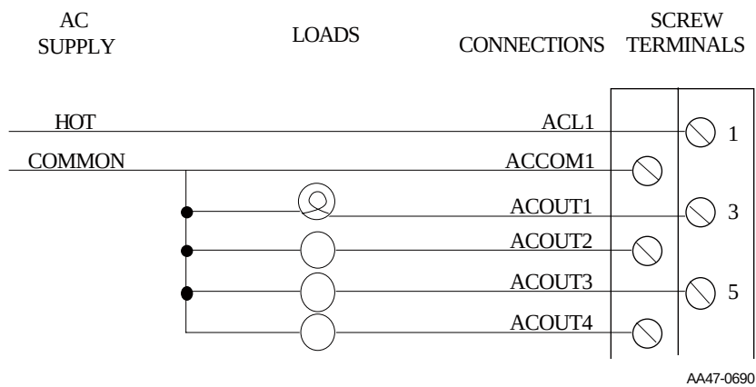
Figure C3-4. Connectors for One Group of Outputs (16 point module)
