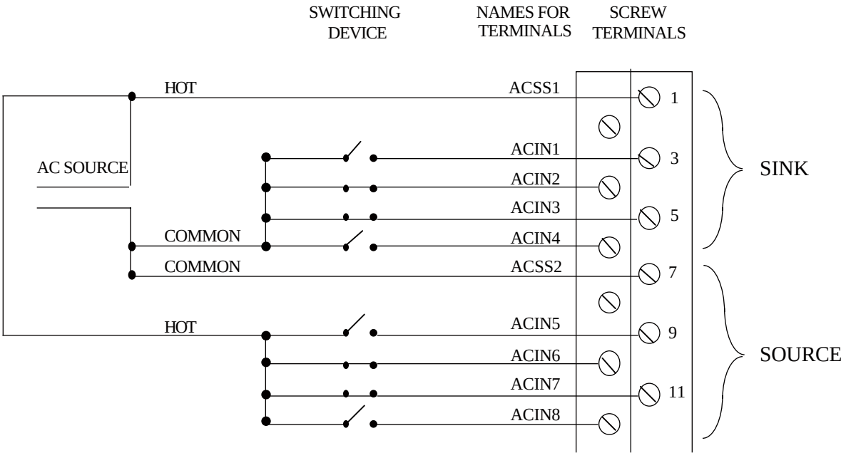
Figure C4-3. Connectors for Two Groups of Inputs
