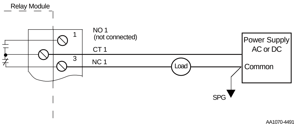
Figure C6-4. Connections for Form C Normally Closed
