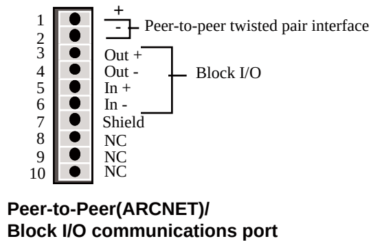
Figure A8-4. Pinout for ARCNET and Block I/O Expansion Port
