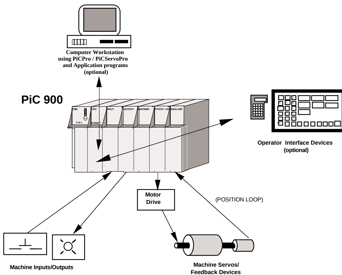
Figure 2. Diagram of the PiC900 system in operation
