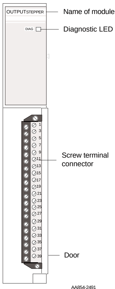
Figure D9-1. OUTPUT STEPPER Axis Module (2, 4, 8 ch)
