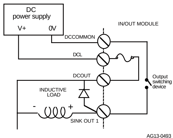
Figure C9-7. Connecting an External Diode
