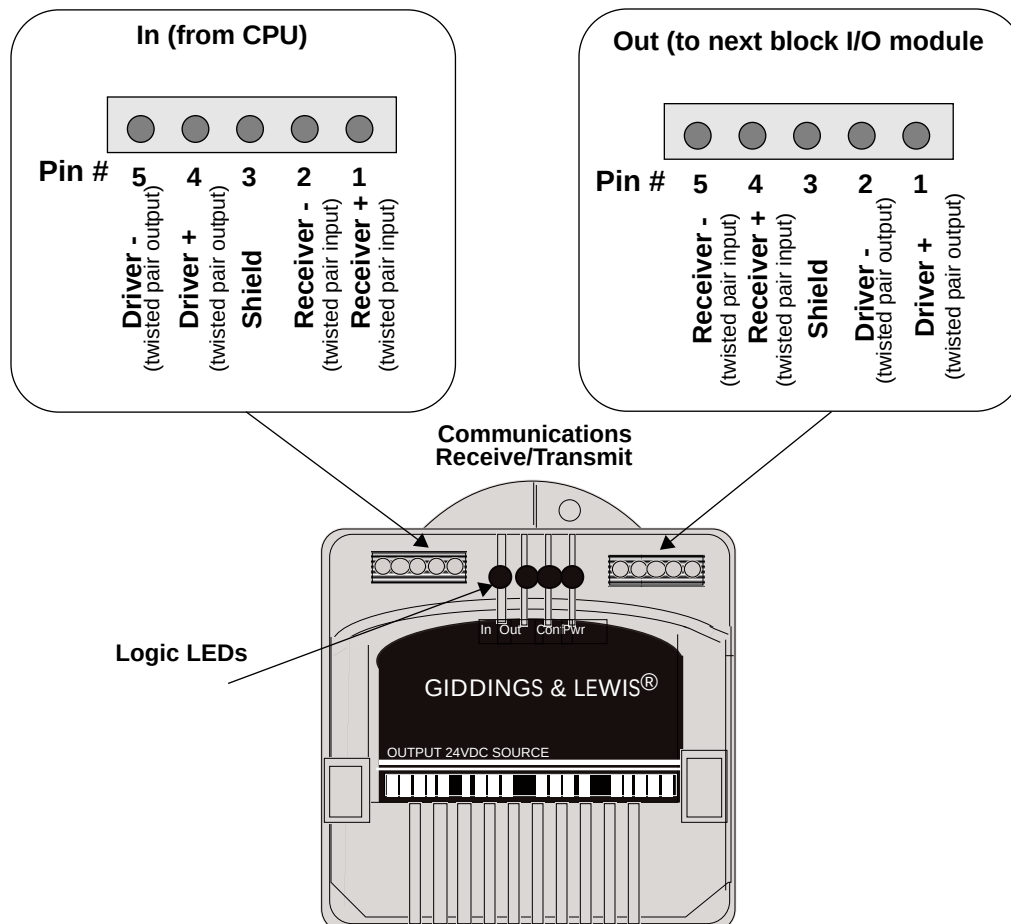
Figure N2-9. Pinouts for Communication Connectors
