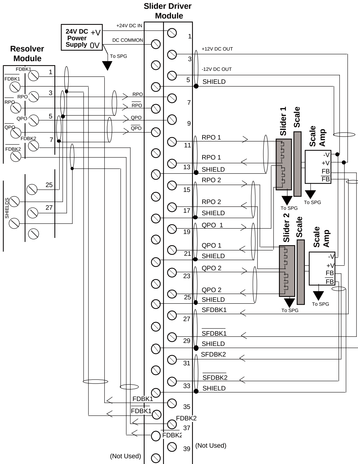
Figure D7-4. Connections to Two Inductosyn Systems
