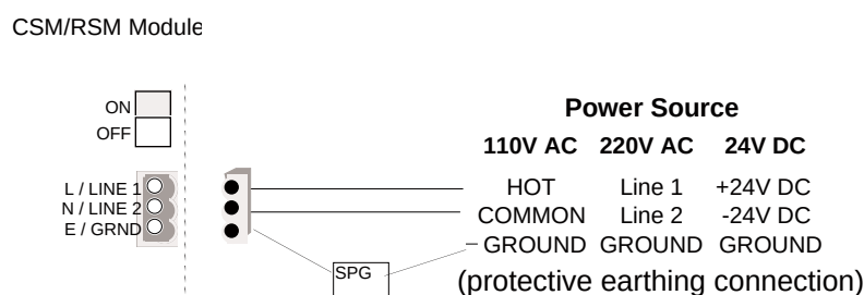
Figure A1-2. Power to the System
