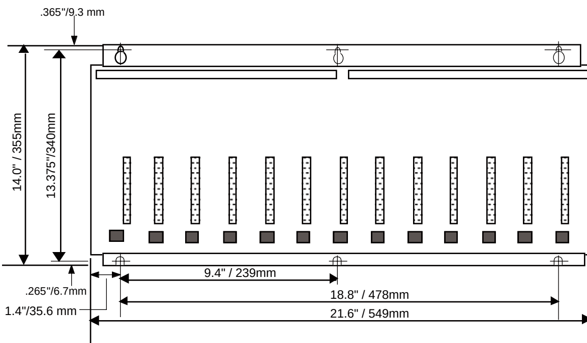
Figure 5. The 13-slot system rack
