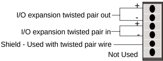
Figure A5-3. Pinout for the I/O driver twisted pair connector
