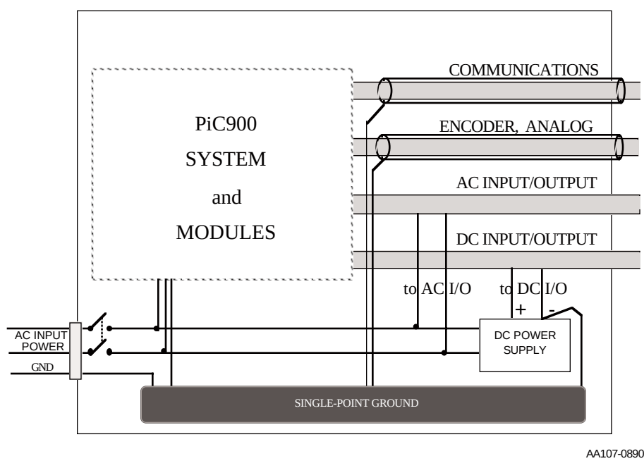
Figure 11. Power and signal cables from the system
