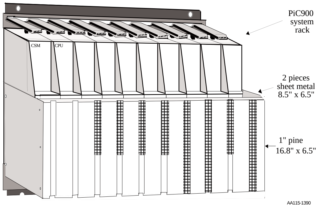
Figure I-1. Jig for Wiring I/O Modules
