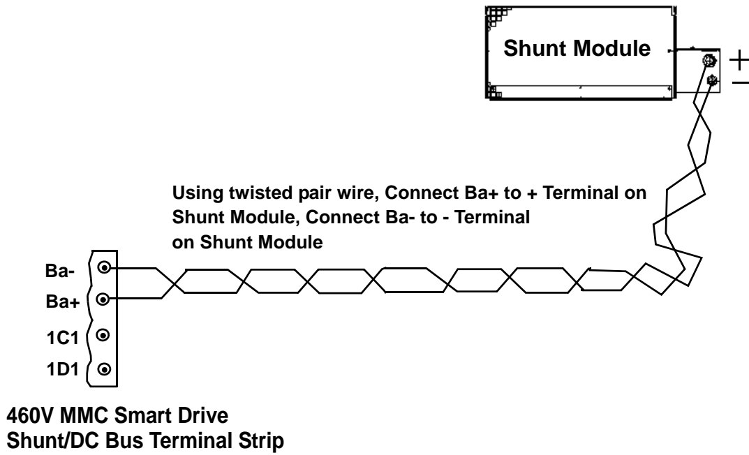
Figure 8-4: Wiring 460V MMC Smart Drive to 2800 Watt, 25Ω Shunt Module / 3900 Watt, 18Ω Shunt Module
