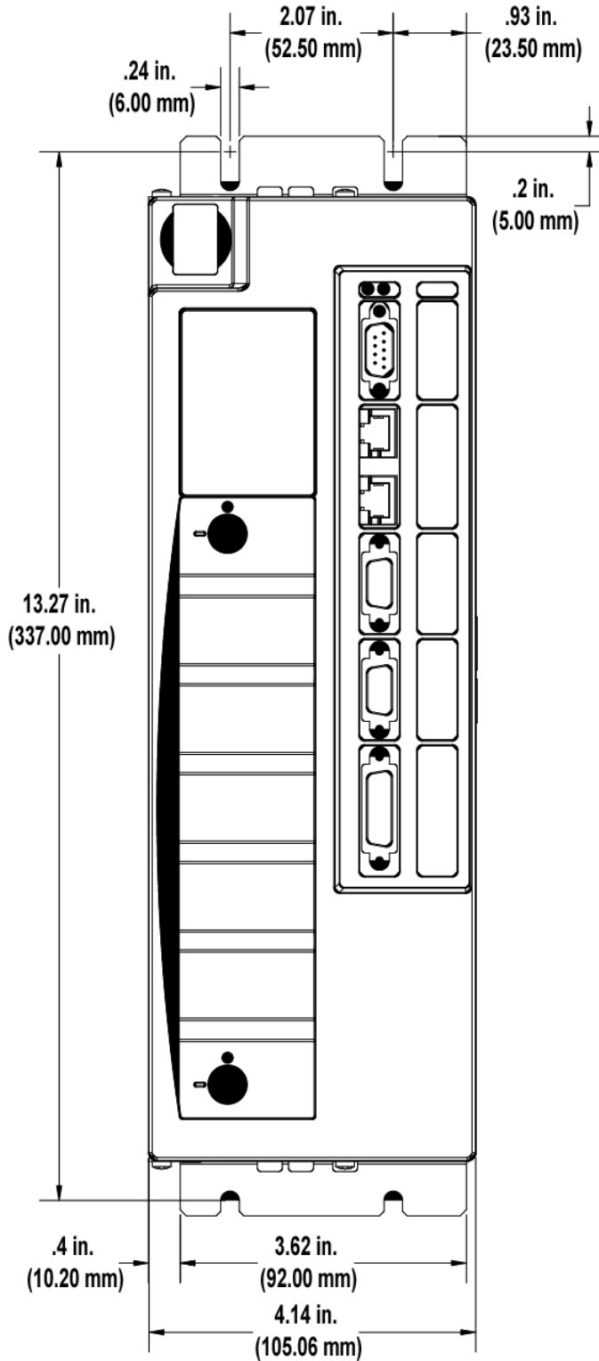
Figure 6-9: Size 1 460V Smart Drive - Front View
