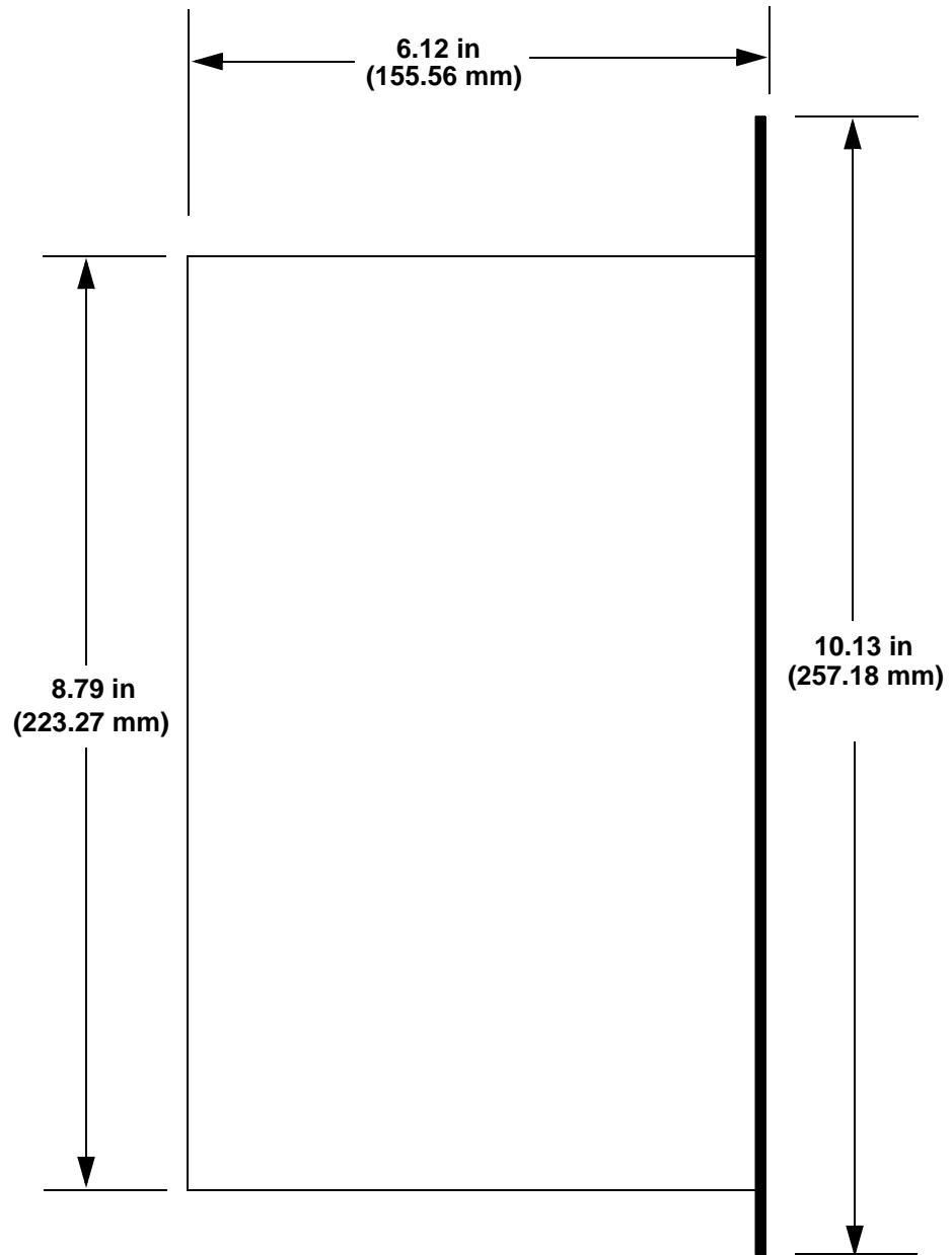
Figure 5-12: 230V Standard (non -DN) and Narrow (-DN) Drive - Side View
