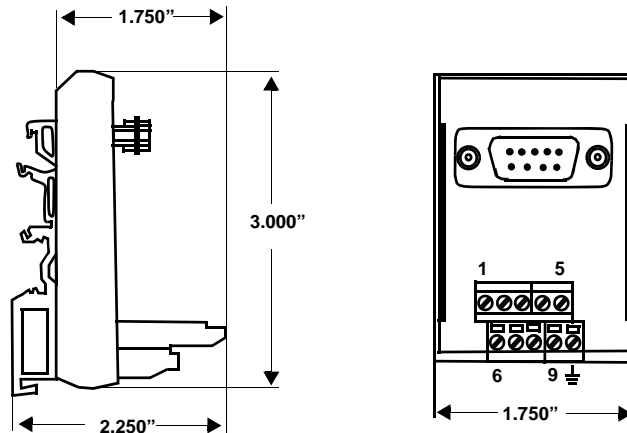
Figure 11-3: Block I/O Breakout Box Dimensions
