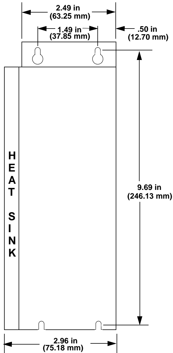
Figure 5-8: 500 W Narrow Drive (-DN) - Front View
