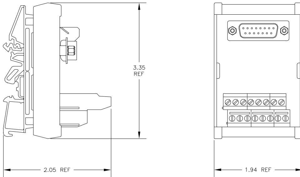
Figure 7-3: Aux Feedback Port Breakout Box Dimensions
