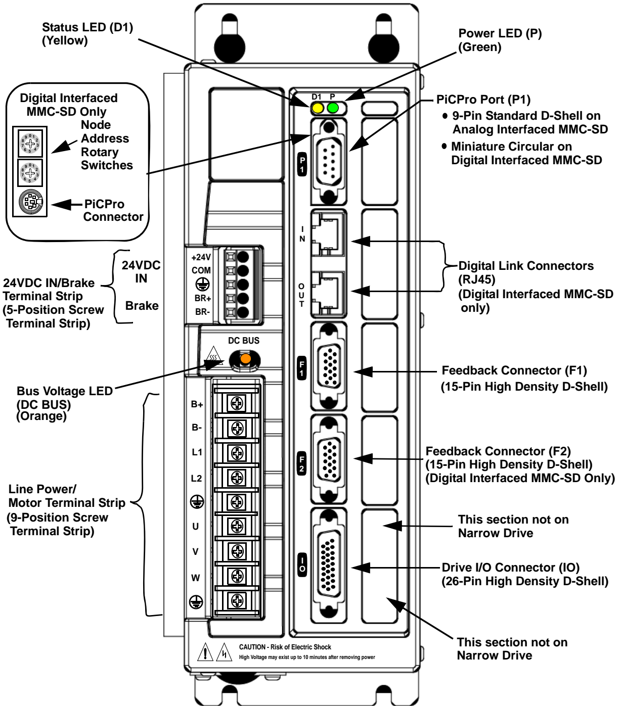
Figure 5-1: Front Panel, 230V Single Phase (500W, 1kW, 2 kW)
