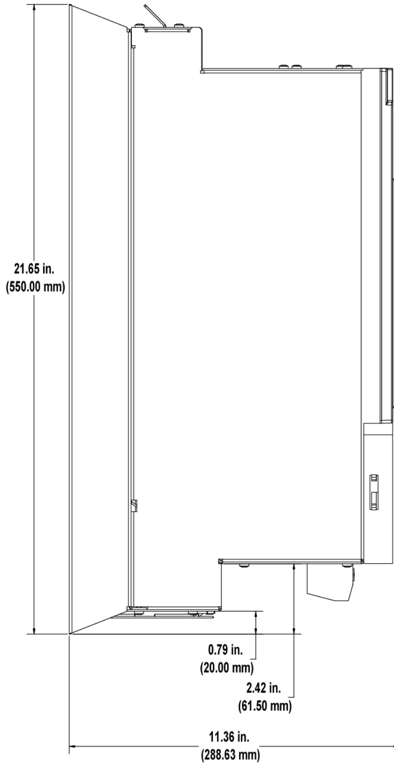
Figure 6-14: Size 3 460V Smart Drive - Side View
