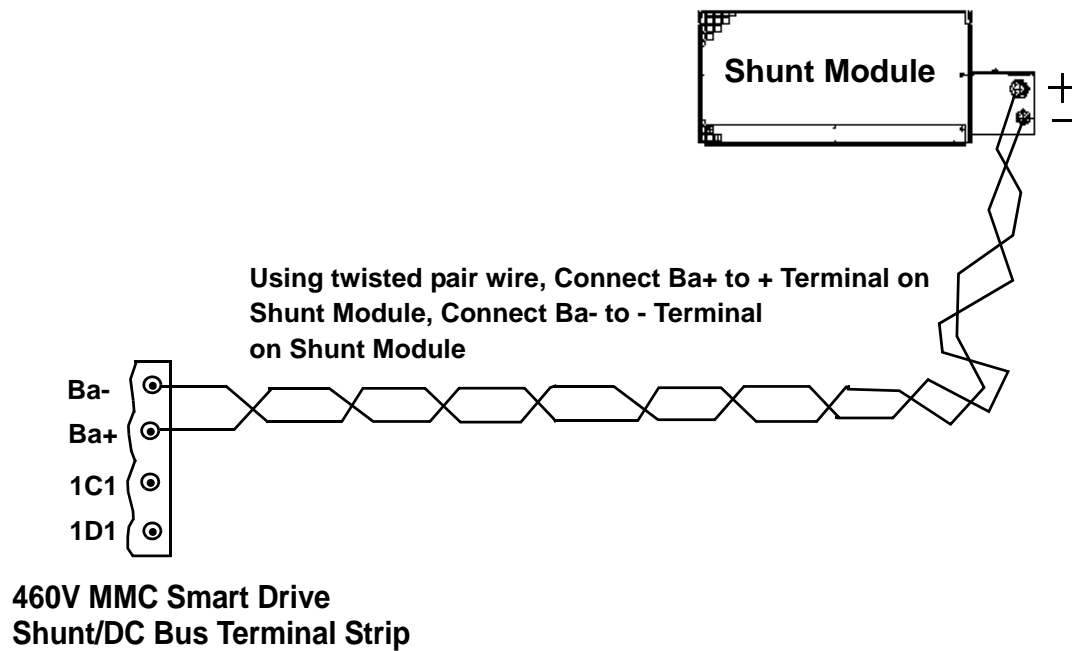
Figure 8-4: Wiring 460V MMC Smart Drive to 2800 Watt, 25 \Omega Shunt Module / 3900 Watt, 18 \Omega Shunt Module
