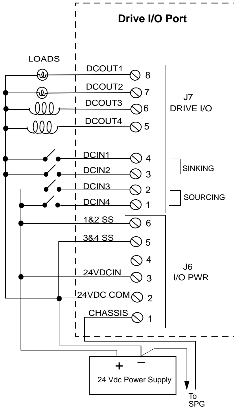
Figure 7-3: Connecting Devices to the Drive I/O Port
