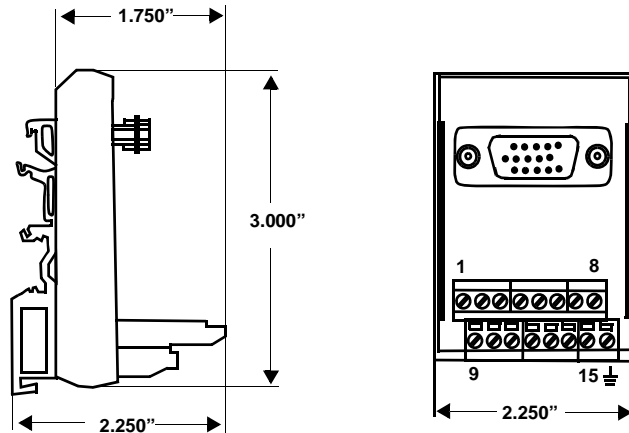
Figure 11-4: User Port Breakout Box Dimensions
