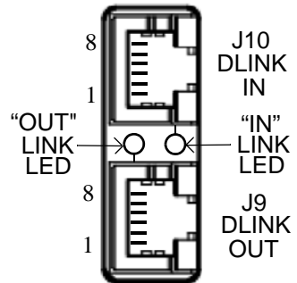
RJ-45 Connectors
