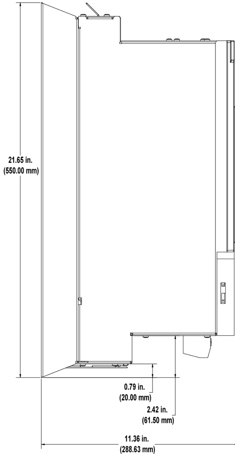
Figure 6-14: Size 3 460V Smart Drive - Side View
