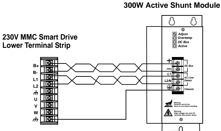
Figure 8-2: Wiring 230V MMC Smart Drive to 300W Active Shunt Module
