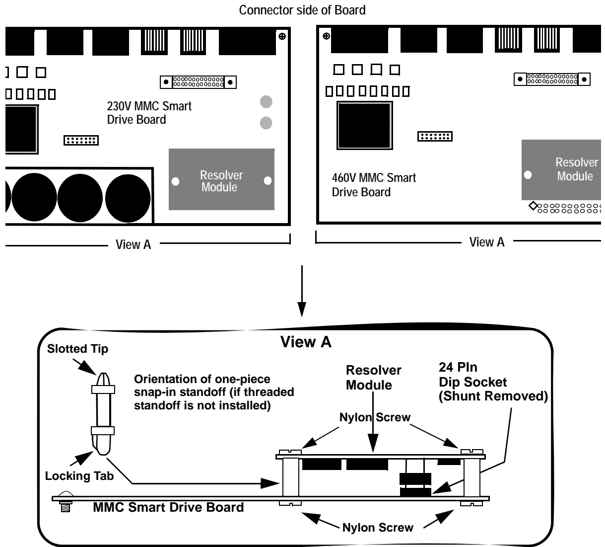
Figure 10-2: : Shunt Removed and Resolver Module Installed
