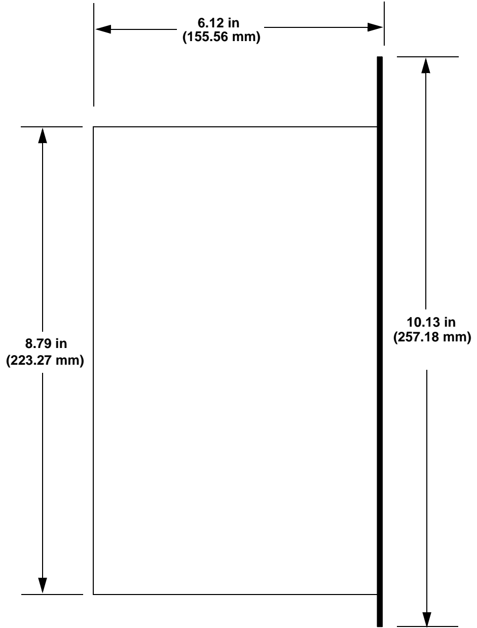
Figure 5-9: 230V Standard (non -DN) and Narrow (-DN) Drive - Side View
