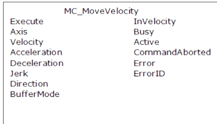
Figure 1-76: MC_MoveVelocity
