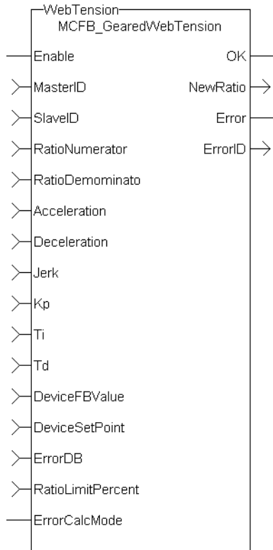
Figure 1-148: MCFB_GearedWebTension Function Block I/O
