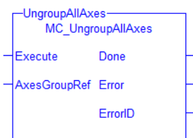
Figure 1-101: MC_UngroupAllAxes
