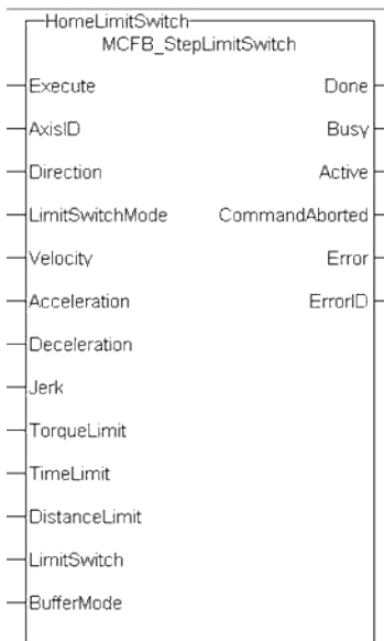
Figure 1-143: MCFB StepLimitSwitch
