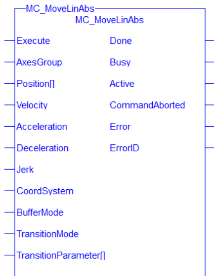
Figure 1-115: MC_MoveLinAbs
