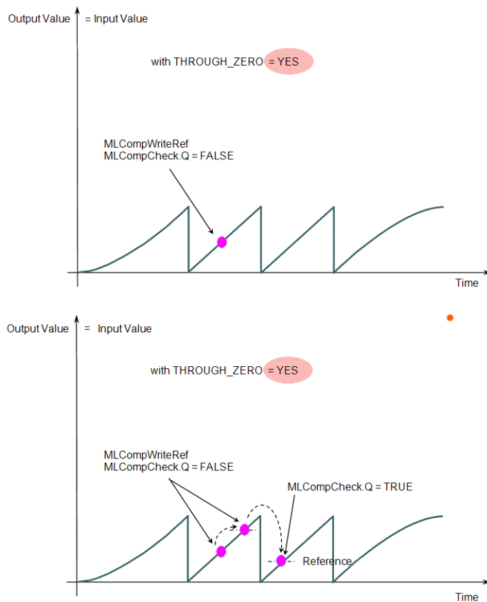
Figure 1-30: Comparator Functions Usage
