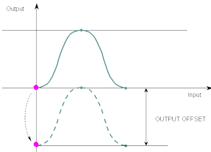
Figure 1-26: MLPrfWriteOOffset
