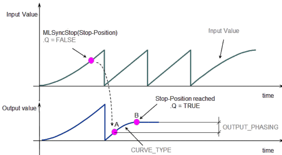
Figure 1-47: MLSyncStop
