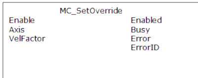
Figure 1-77: MC_SetOverride
