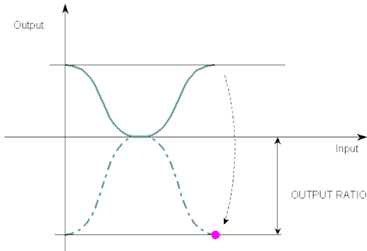
Figure 1-27: MLPfWriteOScale
