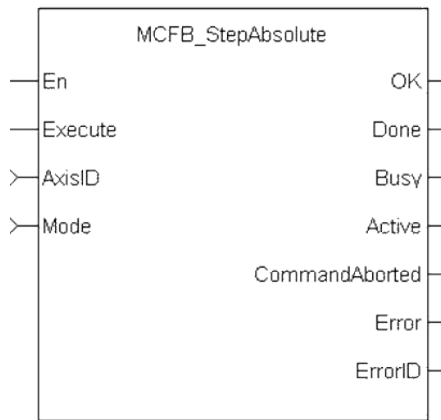
Figure 1-140: MCFB StepAbsolute
