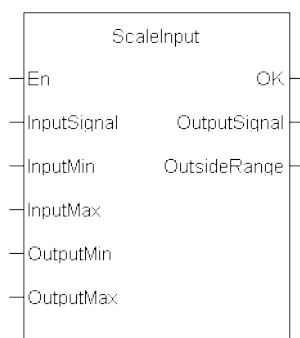
Figure 1-127: Scale Input
