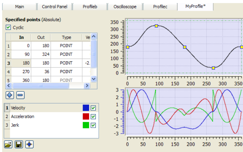
Figure 1-79: MC_CamIn examples
