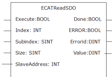
Figure 1-120: ECATReadSdo
