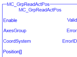
Figure 1-103: MC_GrpReadActPos
