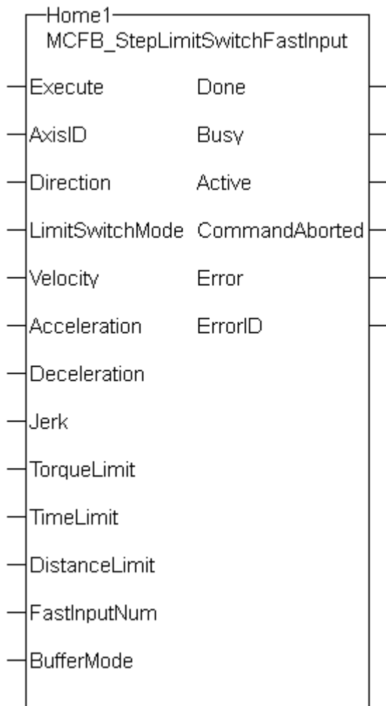
Figure 1-146: MCFB StepLimitSwitchFastInput
