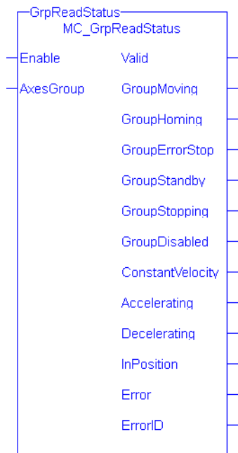
Figure 1-108: MC_GrpReadStatus
