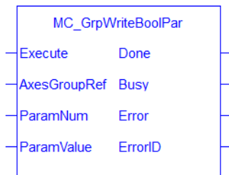
Figure 1-98: MC_GrpWriteBoolPar
