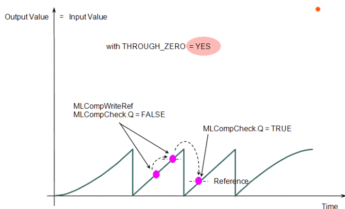
Figure 1-29: MLCompWriteRef
