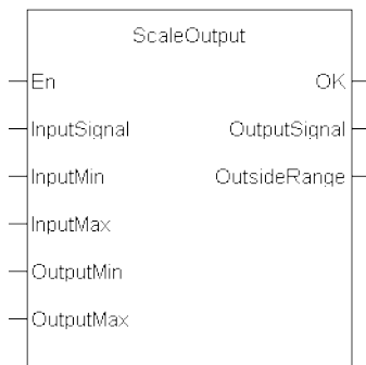
Figure 1-128: Scale Output
