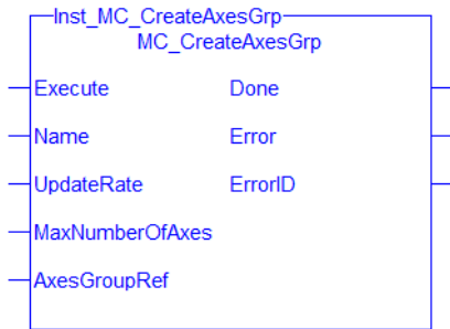
Figure 1-93: MC_CreateAxesGrp
