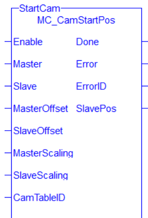
Figure 1-82: MC_CamStartPos
