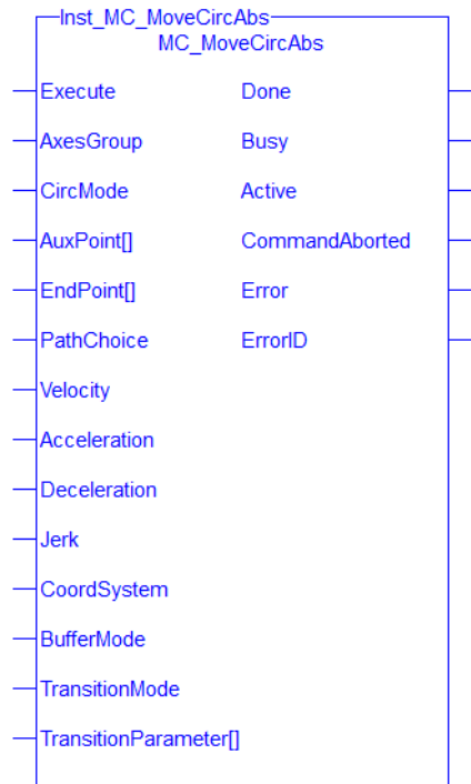
Figure 1-111: MC_MoveCircAbs
