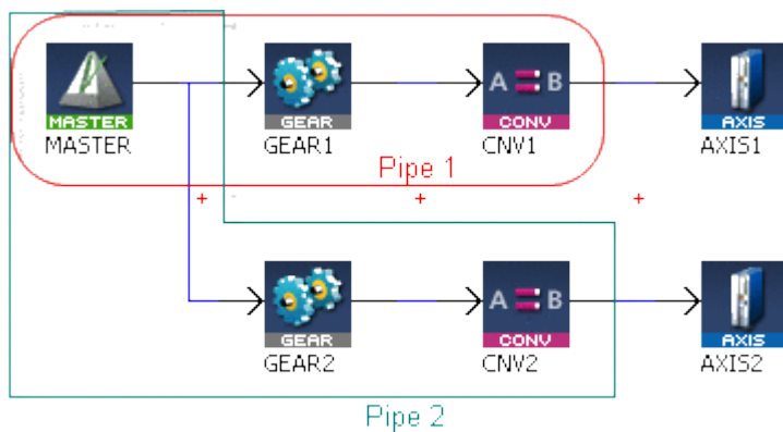
Figure 1-3: MLPipeDeact
