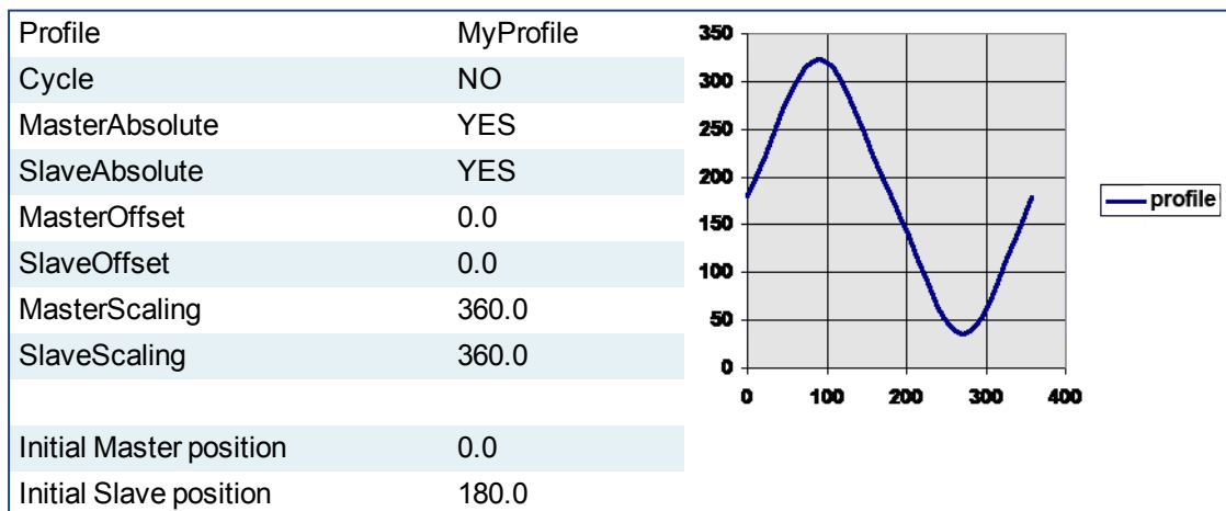
Figure 1-79: MC_CamIn examples
