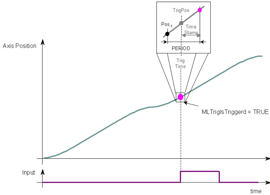
Figure 1-53: MLTrigReadTime
