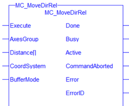
Figure 1-114: MC_MoveDirRel
