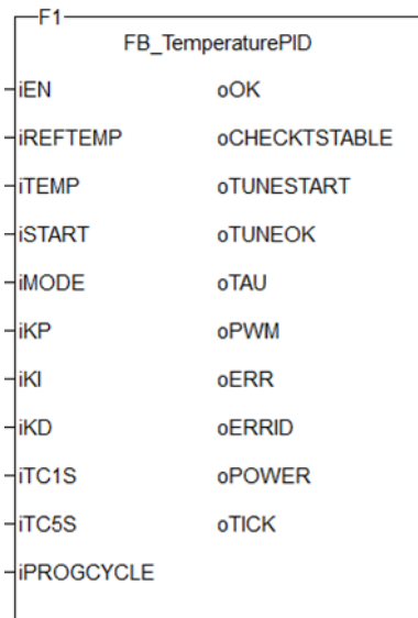
Figure 1-133: The TemperaturePID user-defined function block
