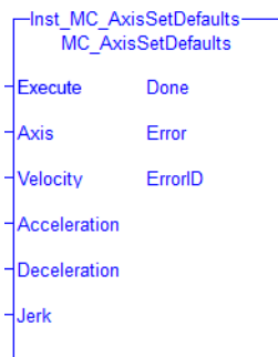
Figure 1-109: MC_AxisSetDefaults
