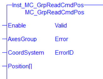
Figure 1-105: MC_GrpReadCmdPos
