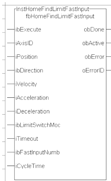
Figure 1-137: MLFB HomeFindLimitFastInput
