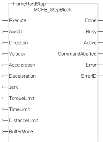
Figure 1-142: MCFB StepBlock
