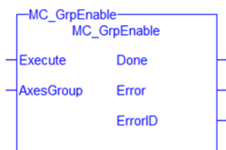
Figure 1-95: MC_GrpEnable
