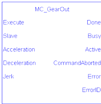
Figure 1-85: MC_GearOut
