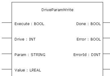
Figure 1-119: DriveParamWrite
