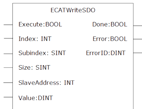
Figure 1-122: ECATWriteSdo
