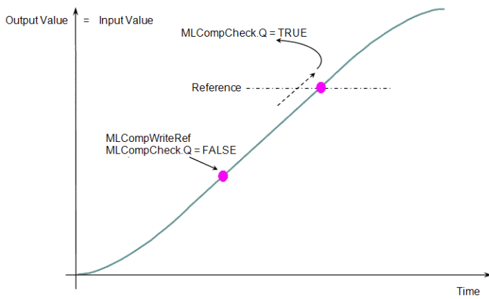
Figure 1-28: MLCompCheck
