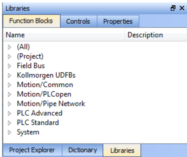
Figure 3-3: Libraries Toolbox
