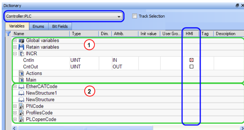
Figure 3-4: Dictionary Toolbox
