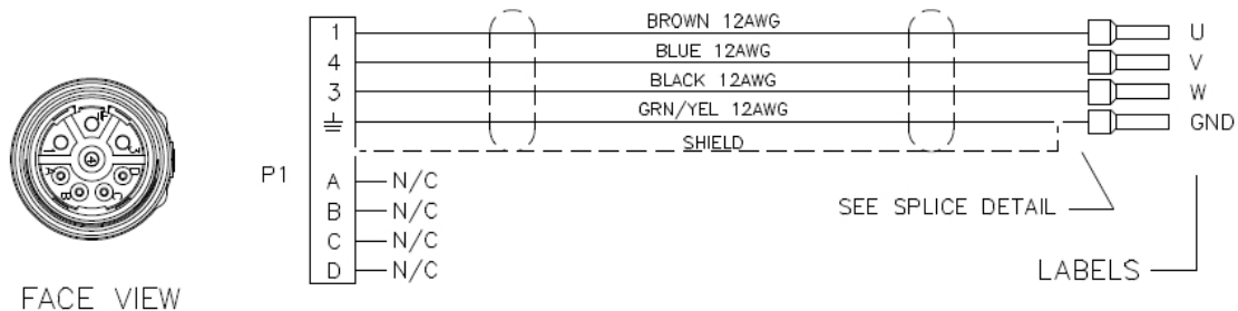
WIRING DIAGRAM
