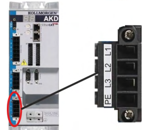
AKD-x02406 & AKD-x00307 a AKD-x02407 (X4)
