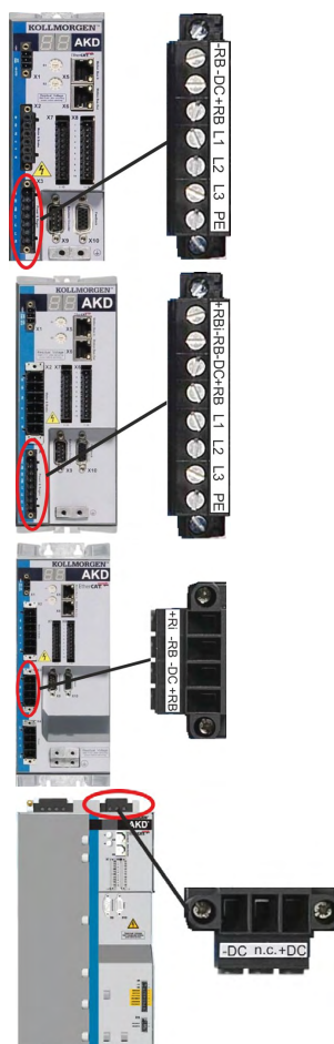
AKD-x00306 a AKD-x00606 (X3)
