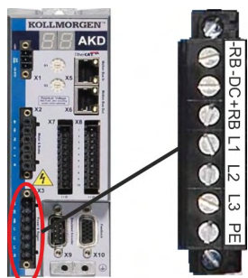
AKD-x00306 a AKD-x00606 (X3)
