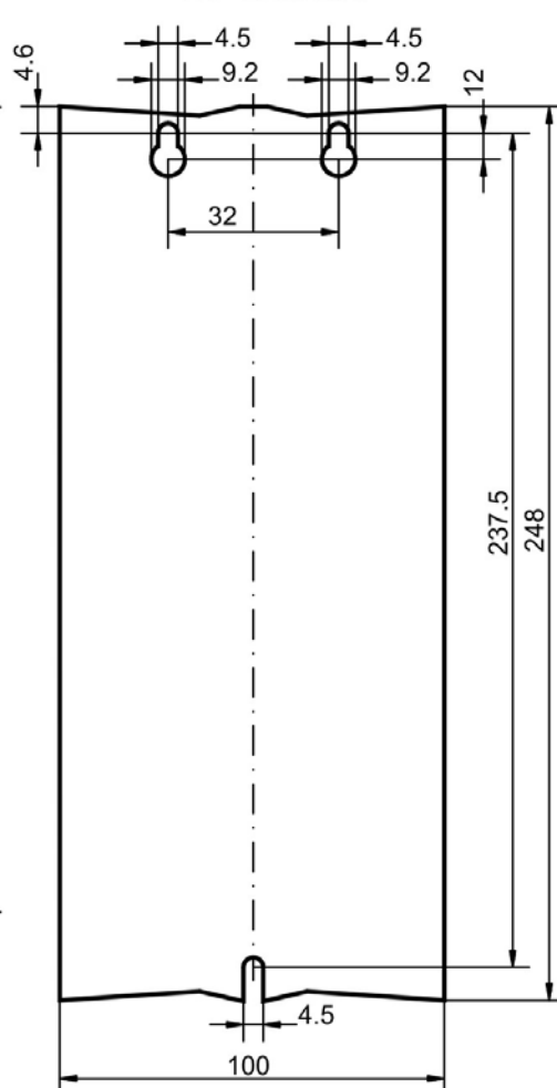
AKD Standard Width 110 - 230V, 24A
