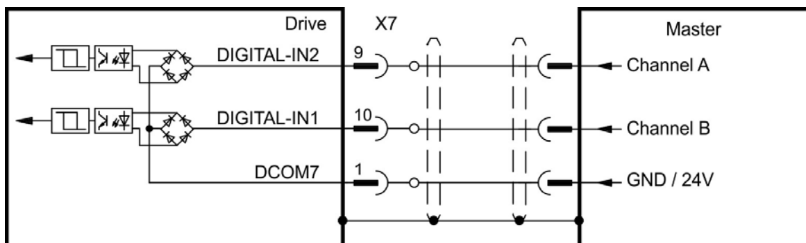
Connection Diagram
