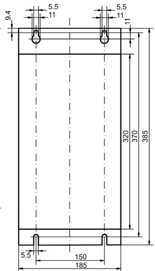
AKD Extended Width 480V, 48A
