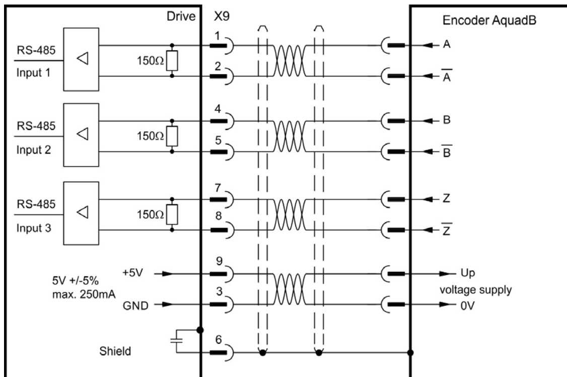
Connection Diagram
