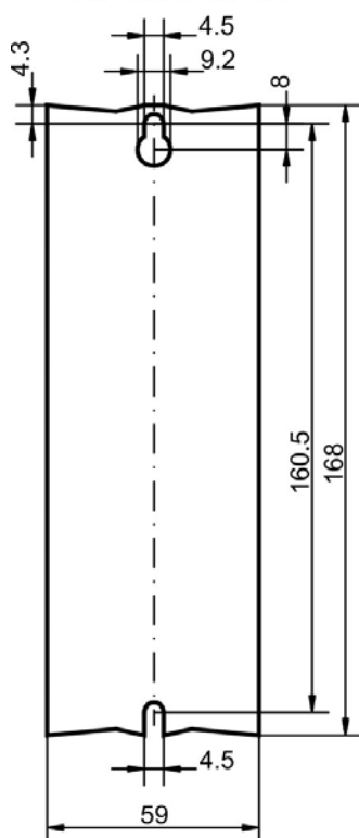
AKD Standard Width 110 - 230V, 3A - 6A
