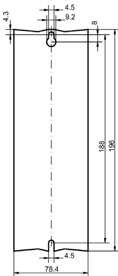
AKD Standard Width 110 - 230V, 12A
