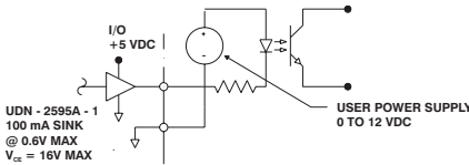
OPTO-ISOLATOR LOAD
