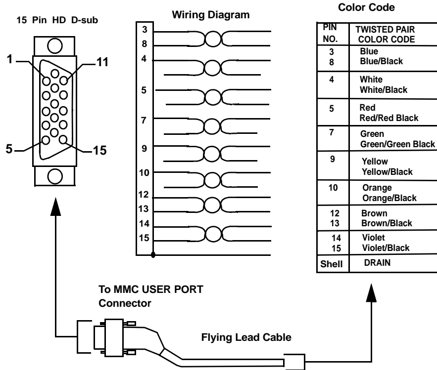
Figure 21-21: Flying Lead Cable to USER PORT Connector
