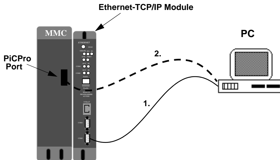
Figure 17-2: MMC/PC Connections
