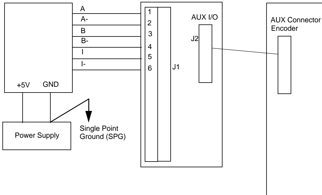
Figure 21-8: Encoder and Power Connections for Encoder Isolator
