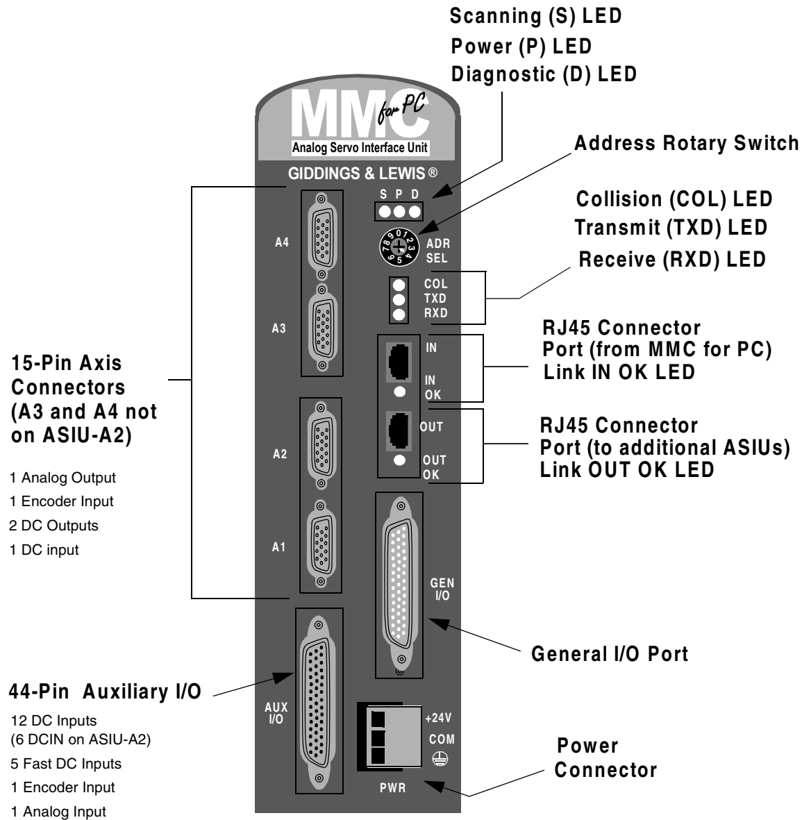
Figure 31: ASIU Components
