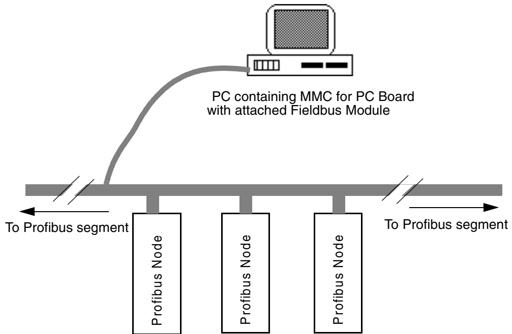
Figure 44: Profibus Connections
