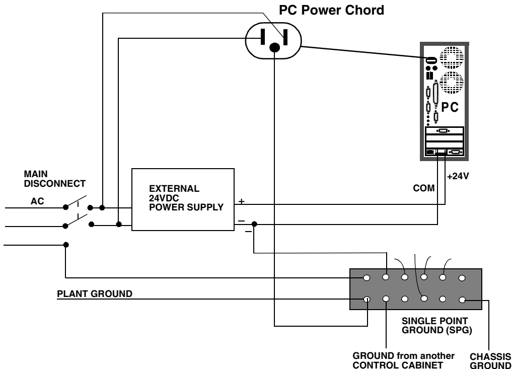
Figure 8: Example of 24 VDC Power Distribution to an MMC for PC System
