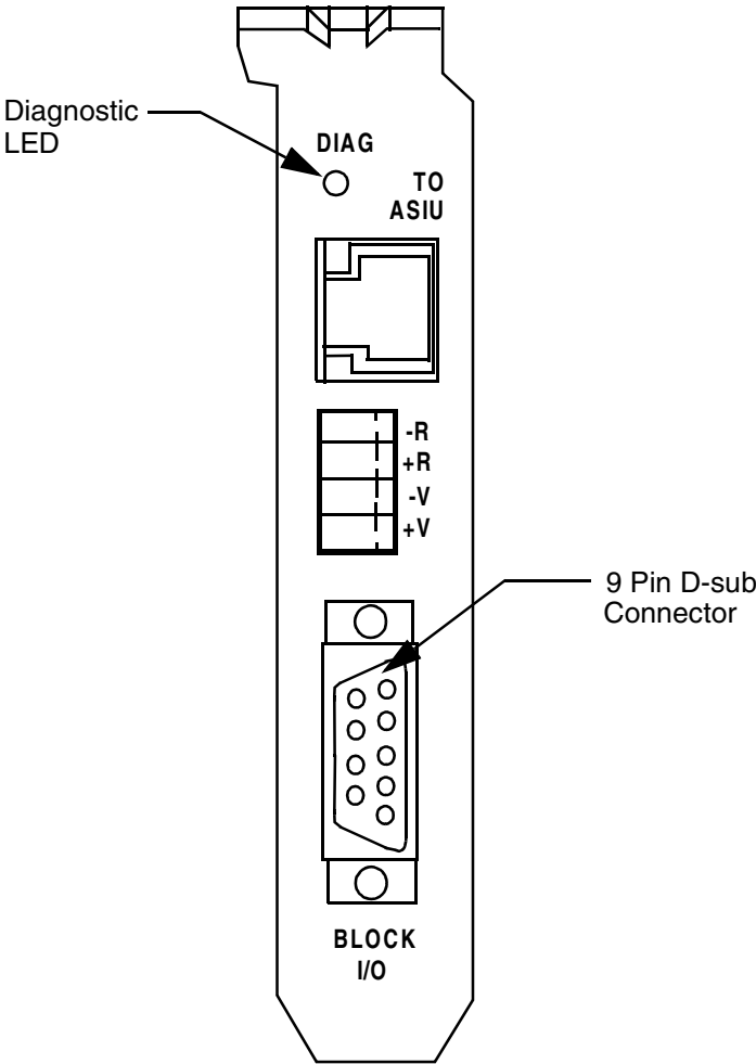
Figure 4: End Bracket Faceplate for Analog Board
