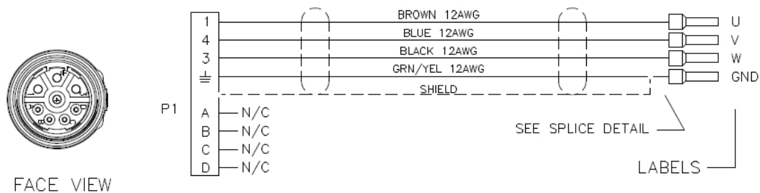
WIRING DIAGRAM
