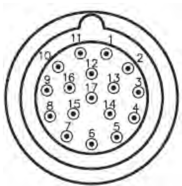
View: solder side of the motor connector.
