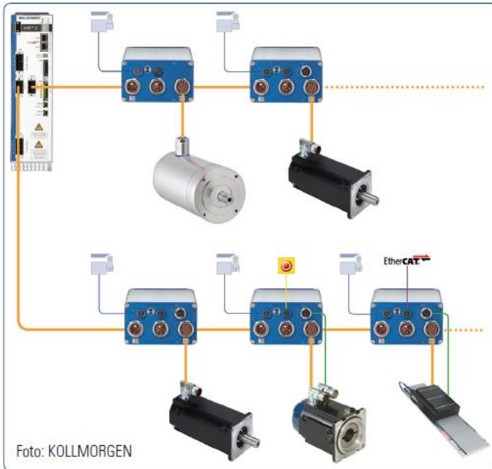
The layout is of distributed servo drive architecture with AKD-N servo drives, different motor types, and single-cable connection technology.
