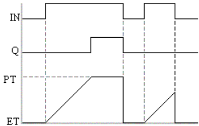
Figure 3-5: Time Diagram
