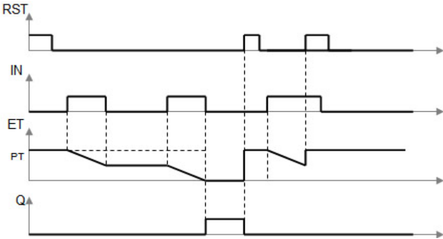
Figure 3-2: Time Diagram
