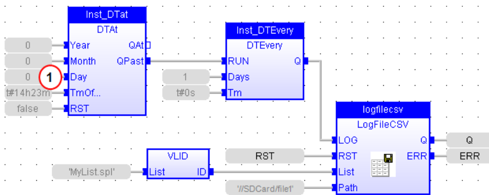
Figure 2-1: Example: LogFileCSV
