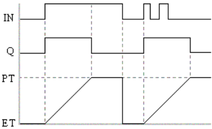
Figure 3-6: Time Diagram
