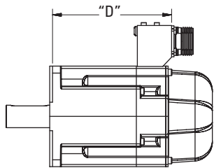
REAR CONNECTOR MOUNTING OPTION
