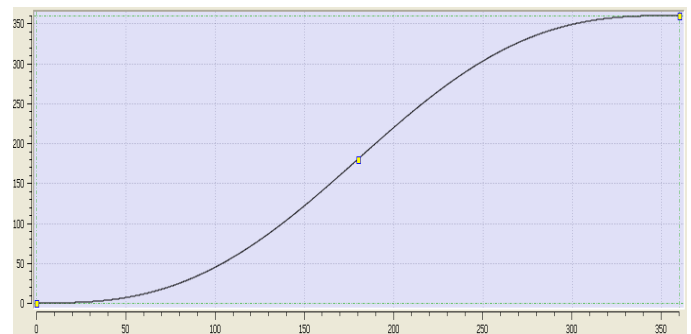
Figure 10: Filling screw base profile
