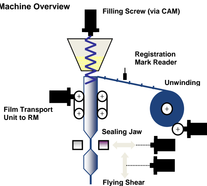
Figure 8: Form, fill and seal machine overview
