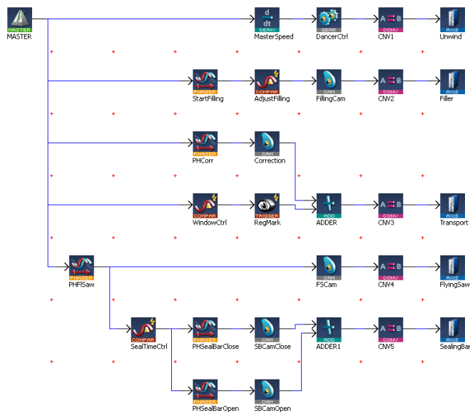
Figure 9: Pipe Network for form, fill and seal machine
