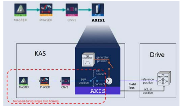
Figure 5: Understanding position data
