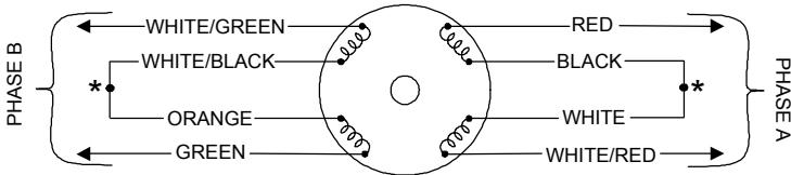
8-LEAD MOTORS, SERIES CONNECTIONS
